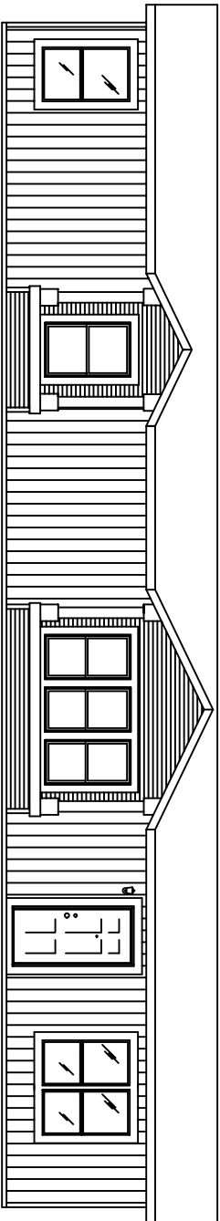
FRONT ELEVATION UPGRADE EXTERIOR
