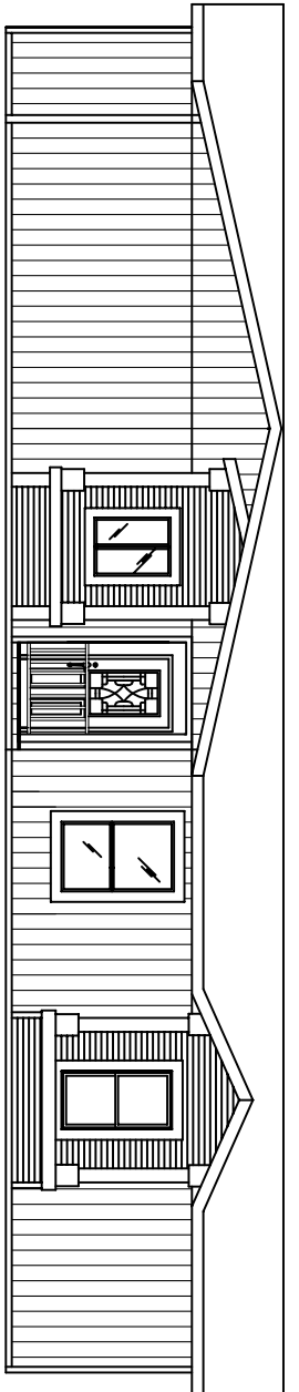
FRONT ELEVATION
