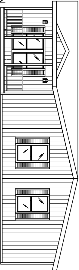
STANDARD EXTERIOR
