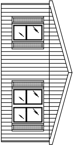
HITCH ELEVATION
